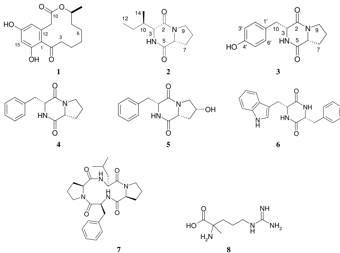
Fig. 1: Isolated compounds of A. versicolour
