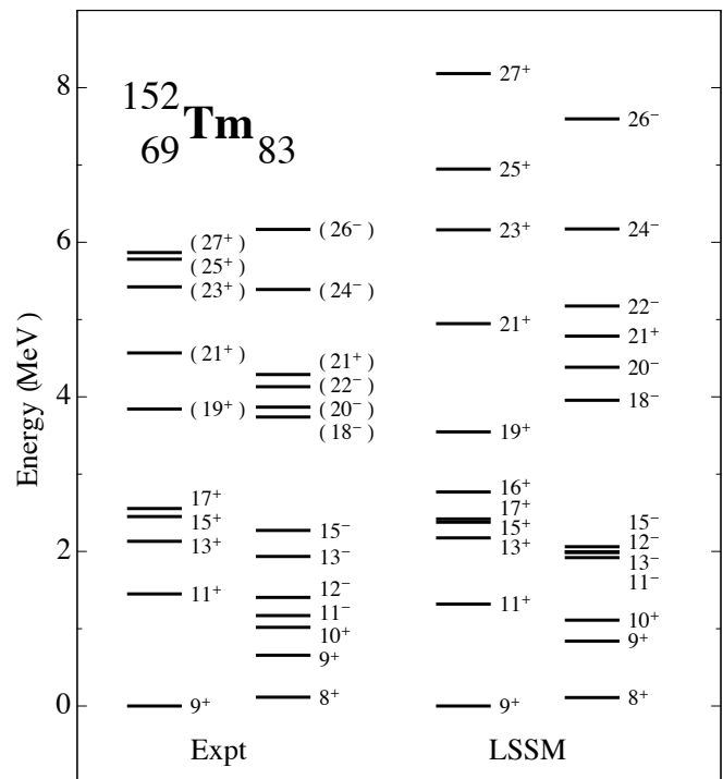
FIG. 8: The observed spectrum of the nucleus ^{152}\text{Tm} (Expt) compared with the results of the full large-scale shell-model (LSSM) calculation. The energy of the 9^+ level is set to zero.
