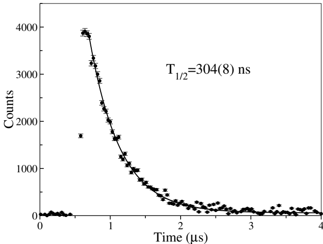
FIG. 3: The time distribution of the \gamma rays, that are marked with asterisks in Fig. 2(b), following the decay of the 17^+ isomeric state in ^{152}\text{Tm} . The solid line is an exponential fit to the data in the range between 0.8 and 2.8 \mu\text{s} .
