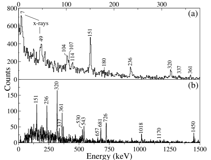
FIG. 4: Delayed \gamma -ray spectra measured by (a) the planar and (b) focal-plane Ge detectors with a time condition that the events should be recorded within 1 \mu\text{s} after the fusion evaporation reaction and in coincidence with the newly observed prompt \gamma -ray transitions in ^{152}\text{Tm} with energies of 128-, 158-, 264-, 287-, 358-, 423-, 439-, 725-, 855-, 1184-, and 1289-keV.
