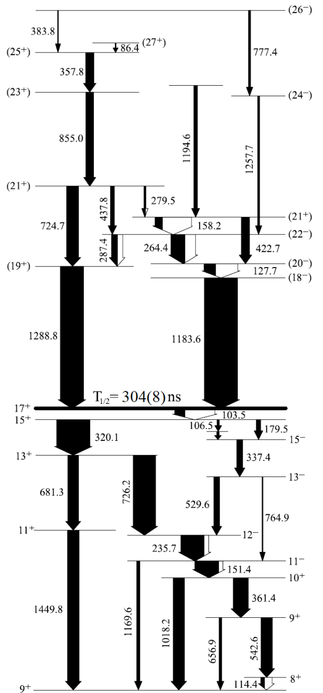
FIG. 1: The deduced level scheme for ^{152}\text{Tm} , including the newly observed levels above the known 17^+ isomeric state. Arrow widths are proportional to relative intensity, and unshaded portions represent the amount of internal conversion. The known level scheme below the 17^+ isomeric state [4] is confirmed from an analysis of the focal-plane data. See the text for more details.
