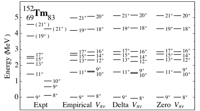
FIG. 10: The observed positive-parity spectrum of ^{152}\text{Tm} (Expt) compared to the results of three different calculations with empirical, delta, and zero proton-neutron interactions in the (\pi 0h_{11/2})^5 \nu 1f_{7/2} model space (see the text for details).
