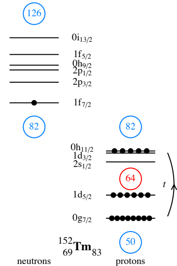
FIG. 7: The model space and the principle of the truncation as used in the large-scale shell-model calculation for ^{152}\text{Tm} . Shell closures are indicated in blue and the subshell closure at Z = 64 is shown in red. The number of protons excited across the Z = 64 subshell closure is denoted as t . As the \pi 0h_{11/2} orbital is crucial for the description of high-spin states in ^{152}\text{Tm} , all five protons are schematically placed in this orbital.
