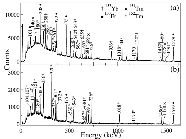
FIG. 2: Focal-plane germanium energy spectra projected from the E_\gamma^D-T_\gamma^D matrix with (a) no time condition and (b) a time condition of T_\gamma^D < 1 \mu\text{s} displaying relative enhancement of the \gamma rays belonging to ^{152}\text{Tm} (see the text for details).
