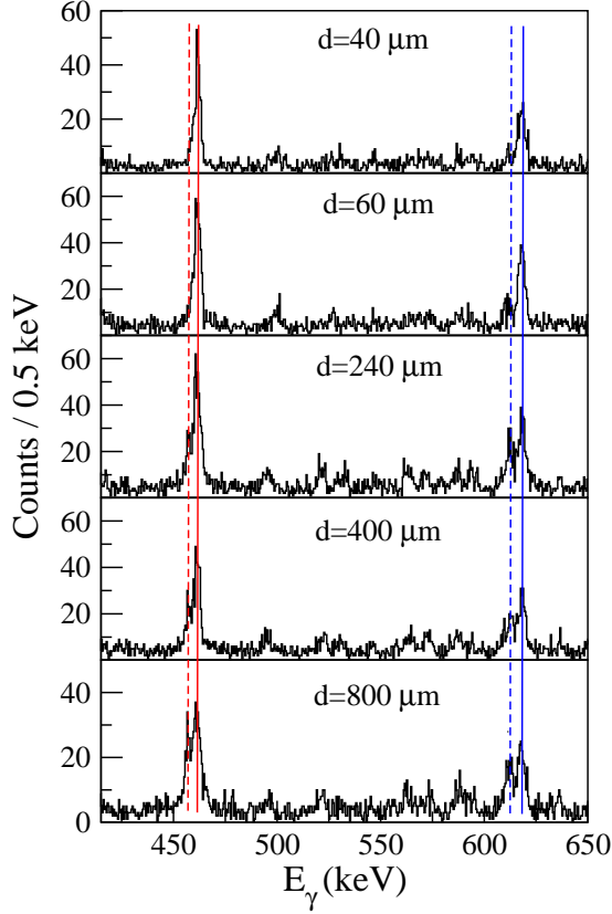
FIG. 1. (Color online) Alpha-decay-tagged \gamma -ray energy spectra used for the lifetime determination in ^{172}\text{Pt} for five different target-to-degrader distances. The centroids for the 2_1^+ \rightarrow 0_{gs}^+ 458 keV \gamma -ray transition when emitted before (after) the degrader foil are indicated by vertical red dashed (solid) lines while the centroids for the 4_1^+ \rightarrow 2_1^+ 612 keV \gamma -ray transition when emitted before (after) the degrader foil are indicated by vertical blue dashed (solid) lines.
