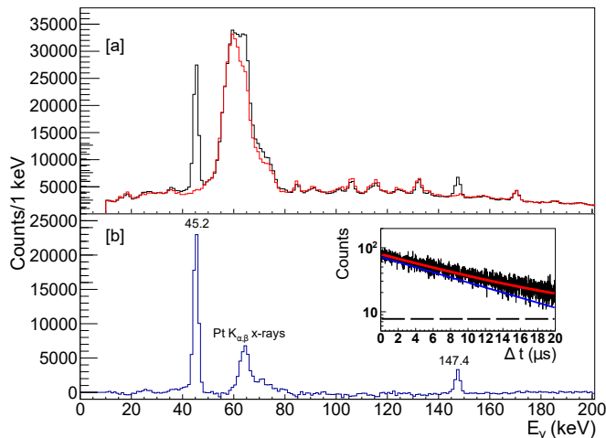
FIG. 1. [a]: Recoil-gated isomeric PGD \gamma -ray energy spectrum observed within 3 – 20 \mu s of the implantation of an ER in the DSSD (black). In red are the time random events observed within a time interval of -5 – 0 \mu s before the recoil implantation and normalised with respect to the black spectrum, based on the ratio of widths of the time intervals. [b]: Background subtracted PGD energy spectrum of \gamma rays observed within 3 – 20 \mu s of the implantation of an ER. The peak at 147.4 keV is a known transition in ^{177}\text{Pt} . The inset shows the decay curve of the 45.2 keV transition together with the fit (in red) which consists of an exponential (in blue) plus a constant background (dashed black).
