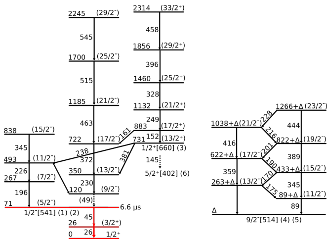
FIG. 3. Simplified partial level scheme of ^{175}\text{Ir} showing states relevant to this work, based on the new data from this study and on the previous decay schemes (cf. Fig. 4 in [4] and Fig. 1 in [3]). For convenience we use the decay energies, to the nearest keV, as deduced by Dracoulis et al. [4], for which our values are in good agreement. All states and transitions above the (5/2^-) state, known from the previous studies, are shown in black; the bands are labelled as per the previous work, K^\pi[N, n_z, \Lambda] in [4] and (1-6) in [3]. The (9/2^-) \rightarrow (5/2^-) transition is unobserved in this work and is shown as a dashed transition. The states and transitions in red show the newly observed 45.2 – 26.1 keV cascade from the 6.6 \mu\text{s} isomeric state. The dashed 145 keV transition from the (13/2^+) state shows schematically the decay to the (5/2^+)[402] band which is unobserved in the IDT spectra. The decay scheme also includes the (9/2^-)[514] band which is unobserved in the IDT spectra.
