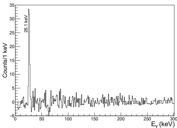
FIG. 4. Background subtracted PGD energy spectrum for \gamma rays in prompt coincidence ( \Delta t(\gamma-\gamma) \leq 50 ns) with the 45.2 keV transition. All events must occur within 3 – 20 \mu\text{s} of an ER implantation in DSSD.
