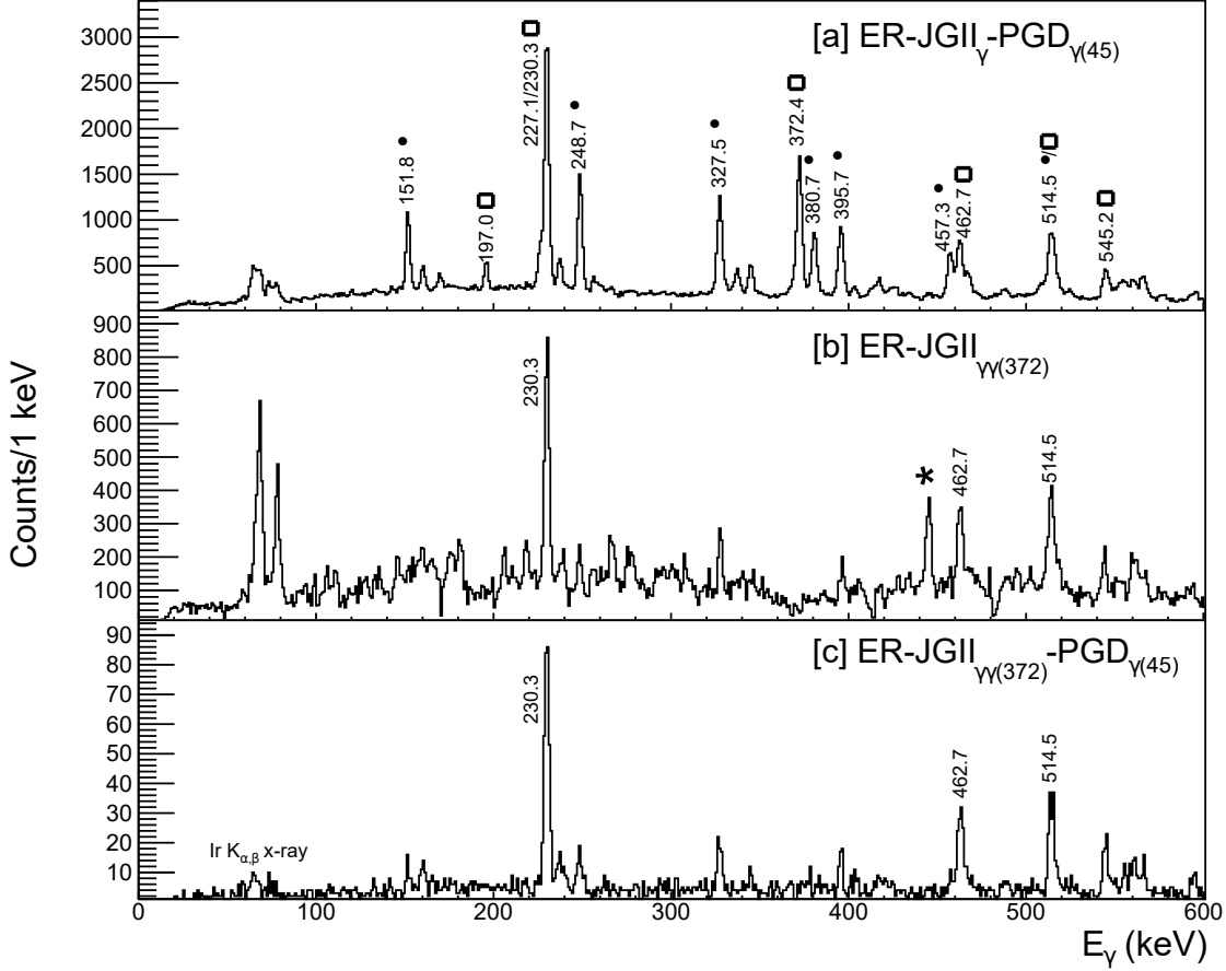
FIG. 2. [a]: Recoil-gated singles JGII \gamma -ray spectrum tagged with the 45.2 keV isomeric transition detected in the PGD. A timing condition of \Delta T(\text{ER-45.2 keV}) = 3\text{--}20 \mu\text{s} was also applied for the PGD. Transitions in the (1/2^+)[660] and (1/2^-)[541] bands are marked with a dot and open box respectively. [b]: Projection of a recoil-gated \gamma - \gamma matrix for events detected in JGII with a gate on the 372.4 keV transition. A contaminant transition is seen at 444 keV and is marked as *. [c]: Same as [b], but tagged on the 45.2 keV transition in the PGD. The transitions used to calculate \alpha_{tot,exp}(45.2) are labelled in the panels [b] and [c].
