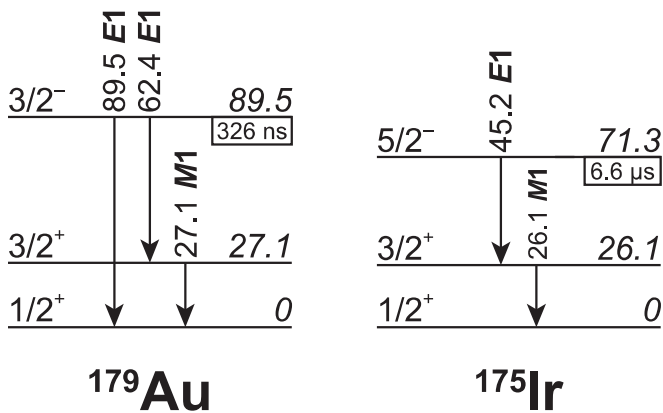
FIG. 5. A comparison of the decay of the 6.6 \mu\text{s} isomer observed in ^{175}\text{Ir} with the decay of a 326 ns isomer in ^{179}\text{Au} [19] showing the similar decay paths.
