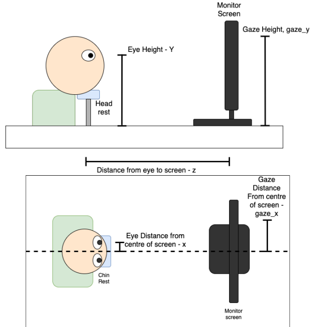
Figure 4: Experimental setup.
