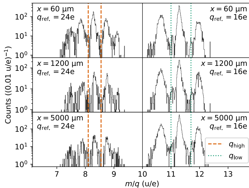
Fig. 6. The mass per unit charge, m/q , distribution of recoils for a selection of plunger distances, for a fixed reference energy of 20 MeV and both q_{\text{ref}} = 16\text{ e} , 24\text{ e} . The limits on the integral of the high and low charge states are shown, which covers the central peak in the DSSD. This peak was chosen as it corresponds to ions which travel down the optical axis of MARA, and so the distribution of energy and charge for these ions correspond to q_{\text{ref}} and E_{\text{ref}} . The ratio of low to high charge state events increases with plunger distance, as is expected.
