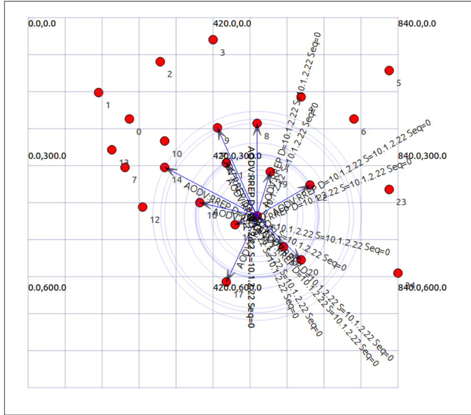
Fig. 1. Initial node position and radio range.
