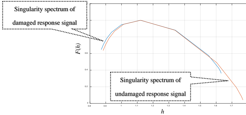
Figure 7. Comparison of singularity spectra from damaged and undamaged structural velocity signal in first floor.
