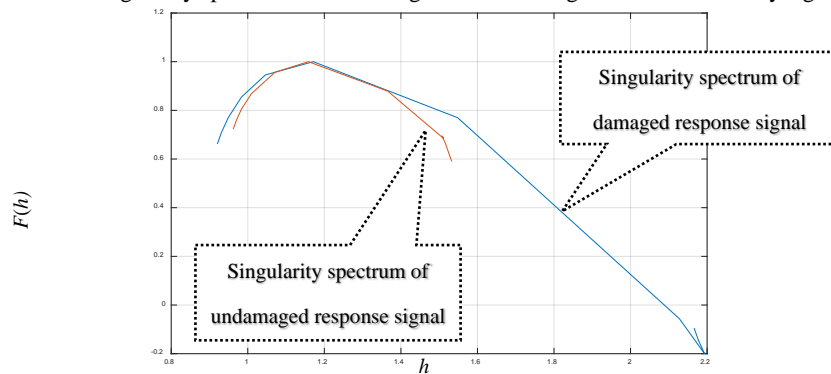
Figure 8. Comparison of singularity spectra from damaged and undamaged structural displacement signal in first floor.
