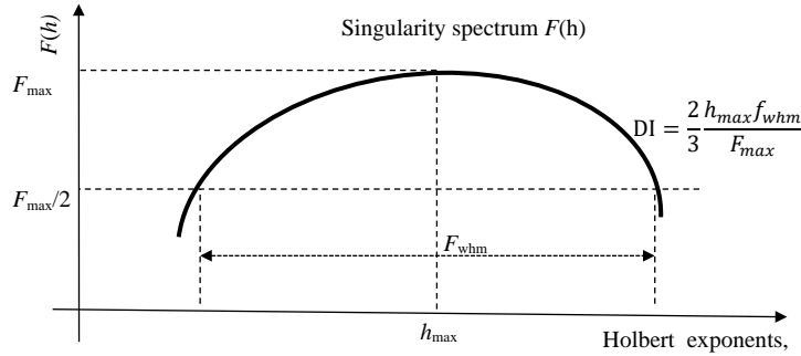
Figure 1. The singularity spectrum, a concave parabolic shape function and representative parameters for calculating the damage indicator.
