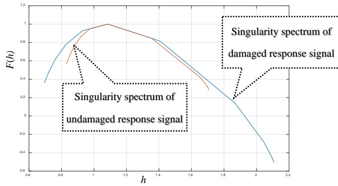
Figure 6. Comparison of singularity spectra from damaged and undamaged structural acceleration signal in first floor.
