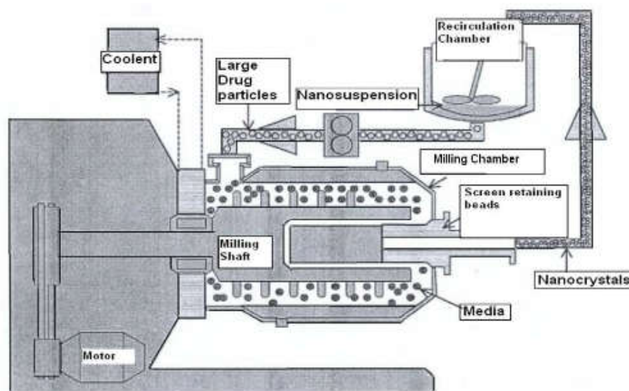
Figure 3. Schematic view of a wet bead milling process [63].
