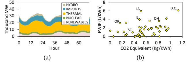
Fig. 2. (a) 3-day fuel mix data of California ISO starting from Sep 1, 2013 [1]. (b) State-level EWIF versus CO 2 emissions in the U.S. [45], [47].
