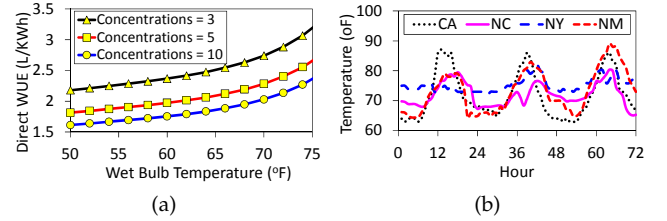
Fig. 1. (a) Direct WUE versus outside wet bulb temperature [44]. Lines/markers represent modeled/measured values. (b) 3-day outside temperature starting from July 1, 2012 [11].
