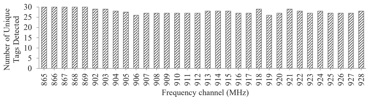
Figure 3. The number of unique tags detected per frequency channel.
