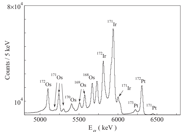
FIG. 1. Total \alpha -particle energy spectrum observed in the DSSDs. Assignments to the main \alpha decay lines are indicated.
