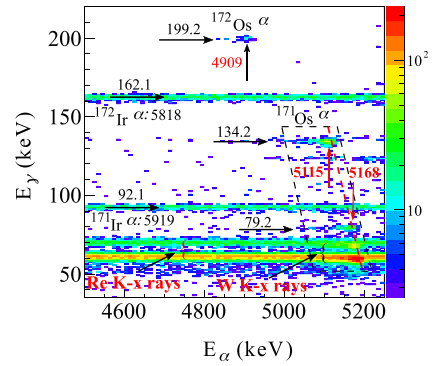
FIG. 4. E_\alpha - E_\gamma coincidence spectrum selected from events with the correlation time interval of < \Delta t(\gamma-\alpha) < 300 ns. All energies are given in keV. Each group is indicated with the corresponding energies and the arrows indicate the positions of the associated \alpha particles and \gamma rays; see details in the text.
