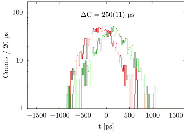
Figure 7. (Color online) Delayed and antidelayed time distribution generated from the 13/2^- \rightarrow 11/2^- \rightarrow 7/2^- cascade. The centroid difference amounts to 250(11) ps.
