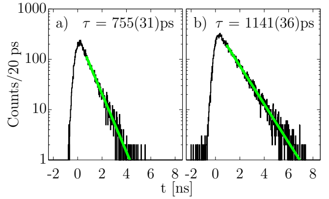
Figure 5. (Color online) Time spectrum for the lifetime measurement of the (a) 9/2^- and (b) 9/2^+ states. (a) Time Spectrum generated by applying a clover gate on the 21/2^+ \rightarrow 17/2^+ (466 keV) transition and placing LaBr gates on the 13/2^- \rightarrow 9/2^- \rightarrow 7/2^- cascade. (b) Time Spectrum generated by applying a clover gate on the 21/2^+ \rightarrow 17/2^+ (418 keV) transition and placing LaBr gates on the 13/2^+ \rightarrow 9/2^+ \rightarrow 9/2^- cascade.
