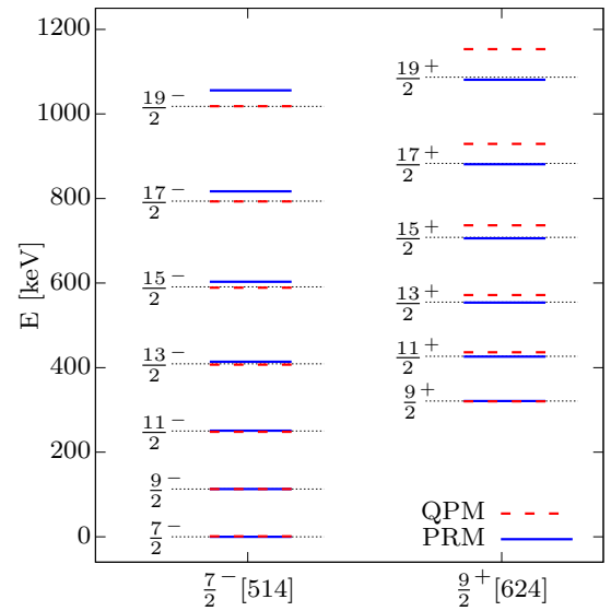
Figure 8. (Color online) Comparison of experimental and calculated level energies. The position of the experimental levels is marked as black (dotted) line and the predictions of the PRM and QPM are shown as blue (dark gray) line and red (dashed) line, respectively.
