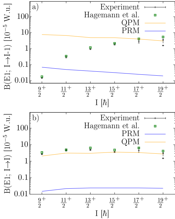
Figure 11. (Color online) Comparison of experimental and theoretical (a) B(E1; I \rightarrow I-1) and (b) B(E1; I \rightarrow I) values. Note the logarithmic scale of the y-axis. The experimental strengths deduced in this work are compared to values gathered by Hagemann et al. [8].
