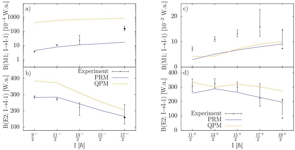
Figure 9. (Color online) Comparison of experimental and calculated B(M1) and B(E2) transition strength for the mixed M1/E2 I \rightarrow I-1 transitions in the (a,b) 7/2^- [514] negative parity band and (c,d) 9/2^+ [614] positive parity band. (a,b) No mixing ratio for the B(M1/E2; 17/2^- \rightarrow 15/2^-) transition is given in the literature. The filled squares give the transition strengths in the limit of pure M1 or E2 transition, respectively.
