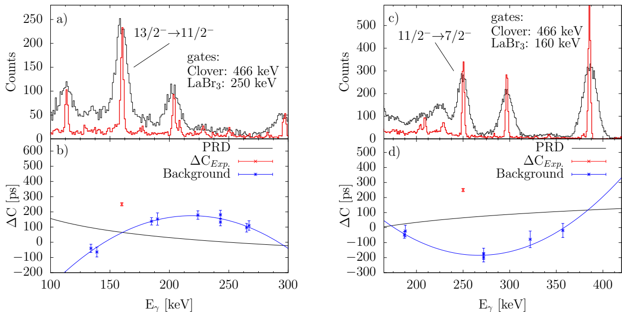
Figure 6. (Color online) Lifetime measurement of the 11/2^- state using the 13/2^- \rightarrow 11/2^- \rightarrow 7/2^- cascade. (a, c) Doubly gated clover and LaBr 3 spectrum with the applied gates indicated in the figures. The peaks corresponding to the feeding and decaying transition of the level of interest are free of any contaminating transition. (b, d) Measured centroid difference (red) and PRD curve (black) shifted to the energy of the applied LaBr 3 gate. In (blue) the measured background time response and corresponding interpolation is shown.
