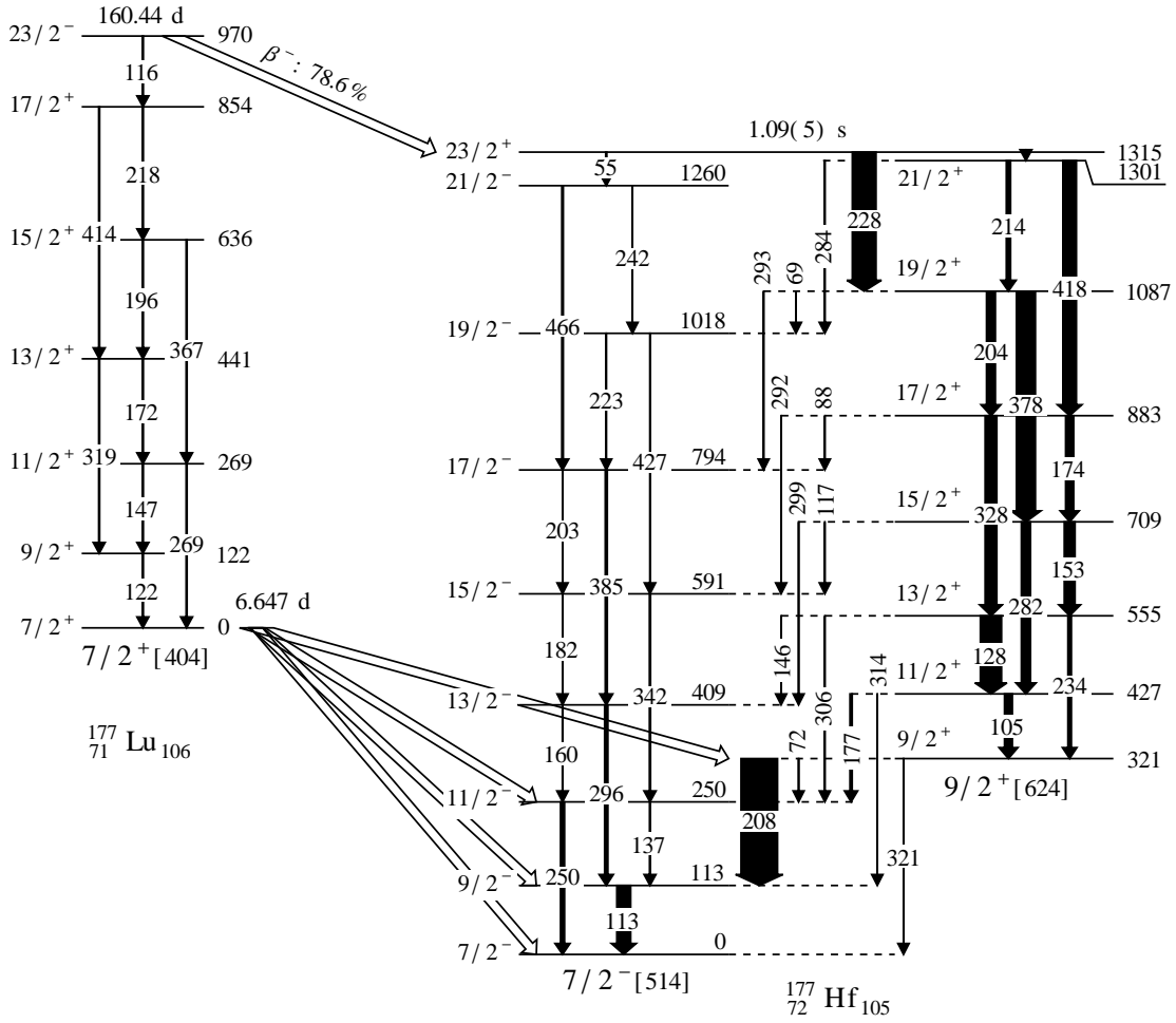
Figure 2. Level scheme of the ^{177m}\text{Lu} decay into ^{177}\text{Hf} . Energies are given in keV and the width of the arrows corresponds to the intensity of the \gamma rays. Adopted from Ref. [12–14]
