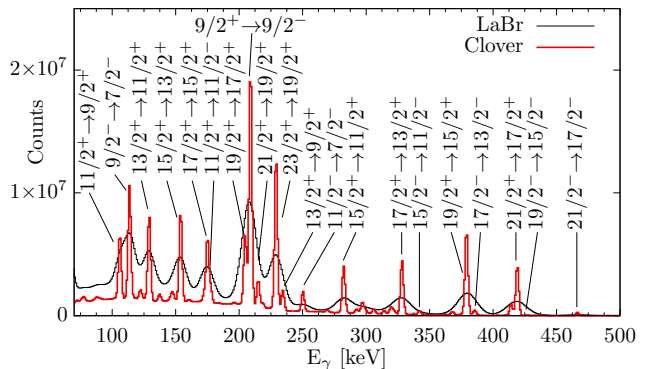
Figure 1. (Color online) Full projections of the clover (red) and LaBr 3 (black) threefold coincidences measured during the 72 h measurement. The clover (LaBr 3 ) spectrum is generated by using Ge-LaBr 3 -Ge (Ge-LaBr 3 -LaBr 3 ) events, respectively. The dominant transitions in 177 Hf are labeled.
