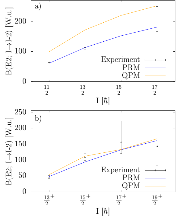
Figure 10. (Color online) Comparison of experimental and calculated B(E2; I \rightarrow I-2) transition strengths in the (a) 7/2^- [514] negative parity band and (b) 9/2^+ [614] positive parity band. Only a lower limit is given for the B(E2; 19^+ \rightarrow 17/2^+) value.
