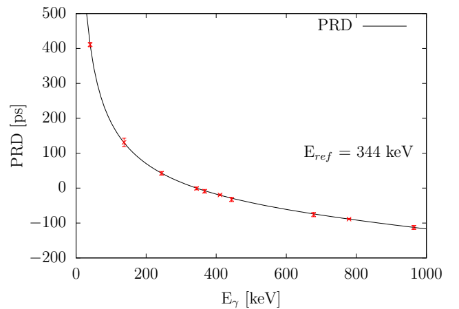
Figure 3. (Color online) Calibrated PRD curve for the EXILL&FATIMA campaign [10] derived using Eq. 3. Due to the low energy of the transitions of interest only the low energy part (below 1 MeV) of the PRD is shown. The uncertainty of the PRD is derived from a 3\sigma standard deviation and amounts to 5 ps.
