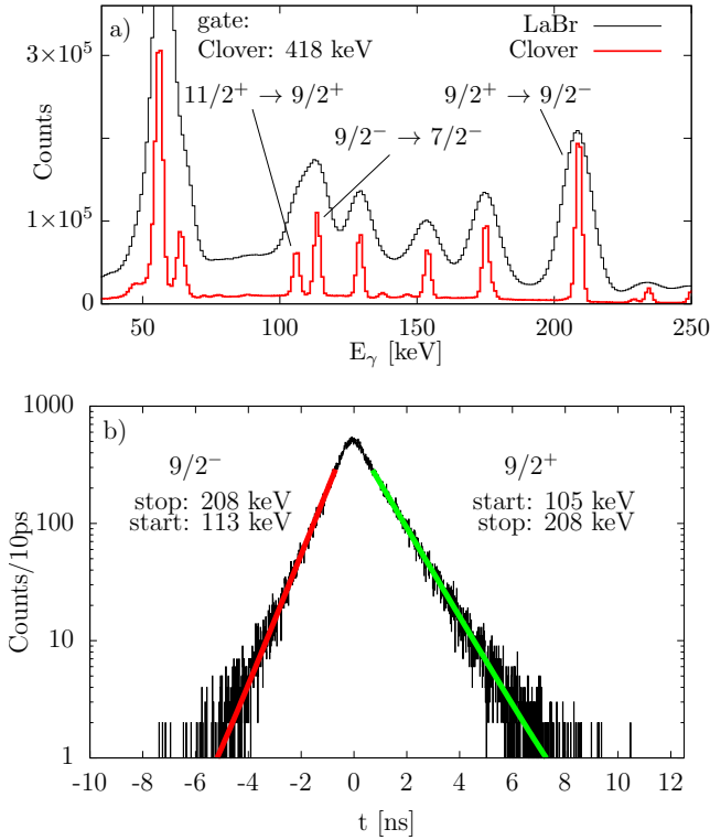
Figure 4. (Color online) (a) Gated spectra after applying a clover gate on the 21/2^+ \rightarrow 17/2^+ (418 keV) transition. This bypasses all contaminations around the 208 keV peak of interest. (b) Time spectrum generated by applying a clover gate on the 21/2^+ \rightarrow 17/2^+ (418 keV) transition, the first LaBr 3 gate on the 9/2^+ \rightarrow 9/2^- (208 keV) transition and a second LaBr 3 gate containing the 11/2^+ \rightarrow 9/2^+ (105 keV) transitions as well as the 9/2^- \rightarrow 7/2^- (113 keV) transition. The lifetimes of the 9/2^+ and 9/2^- states can be measured from the same time distribution.
